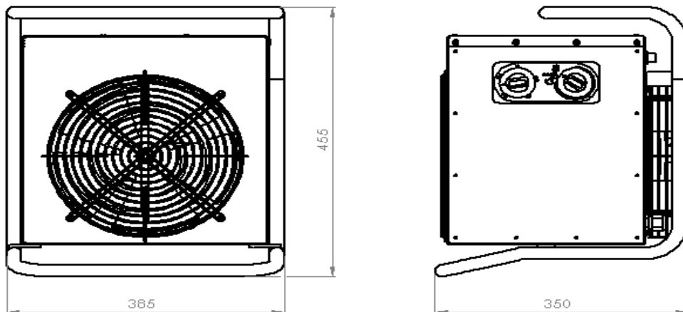
Models FHM 2 - FH 9
